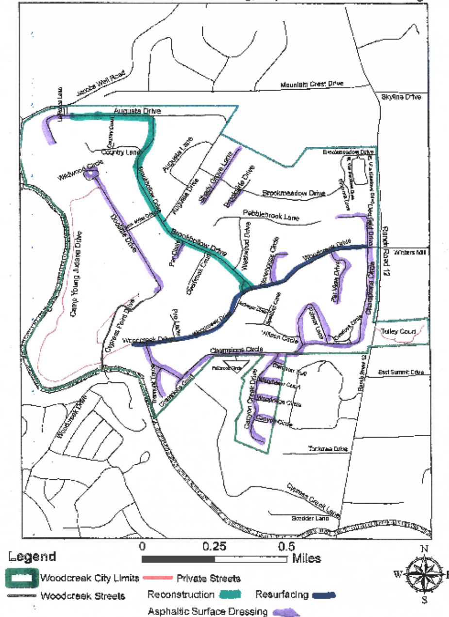
City of Woodcreek Street Map Road Reconstruction, Resurfacing, Asphaltic Surface Dressing
